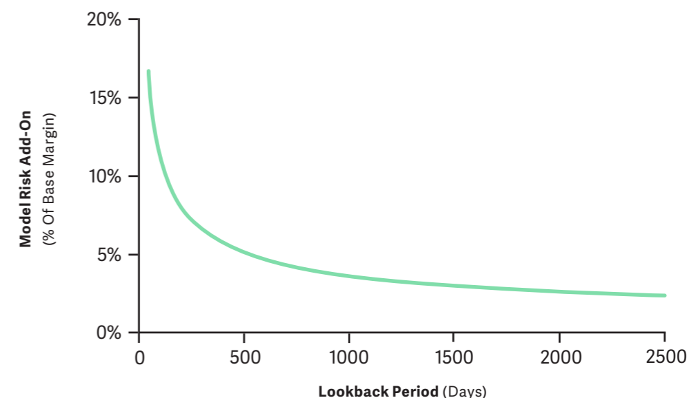
Figure 1. Trade-off between model conservatism and the length of the lookback period
